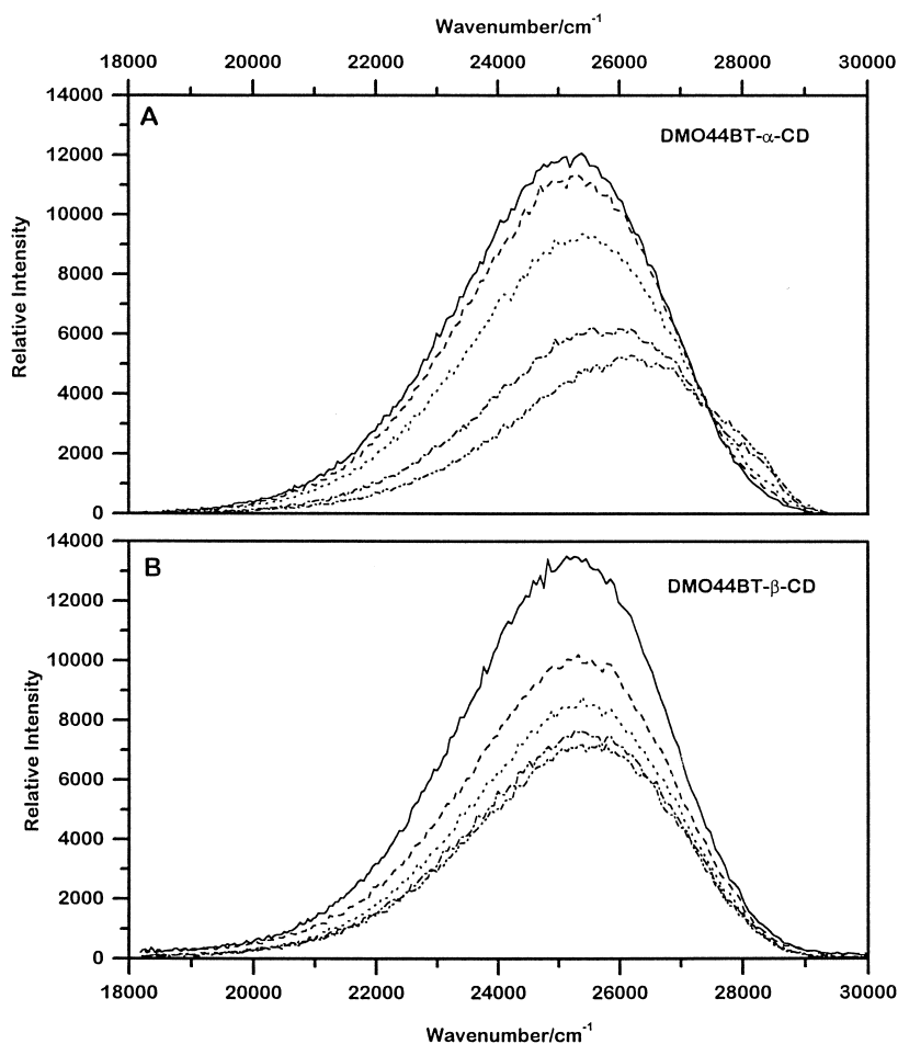
Fig. 1. Fluorescence spectra of DMO44BT in \alpha - and \beta -CD solutions of varying concentrations. (A) [ \alpha -CD] = 0 (solid), 0.30 (dash), 0.75 (dot), 2.00 (dash dot), and 4.00 mM (dash dot dot). (B) [ \beta -CD] = 0 (solid), 0.05 (dash), 0.15 (dot), 0.50 (dash dot), and 2.00 mM (dash dot dot).
