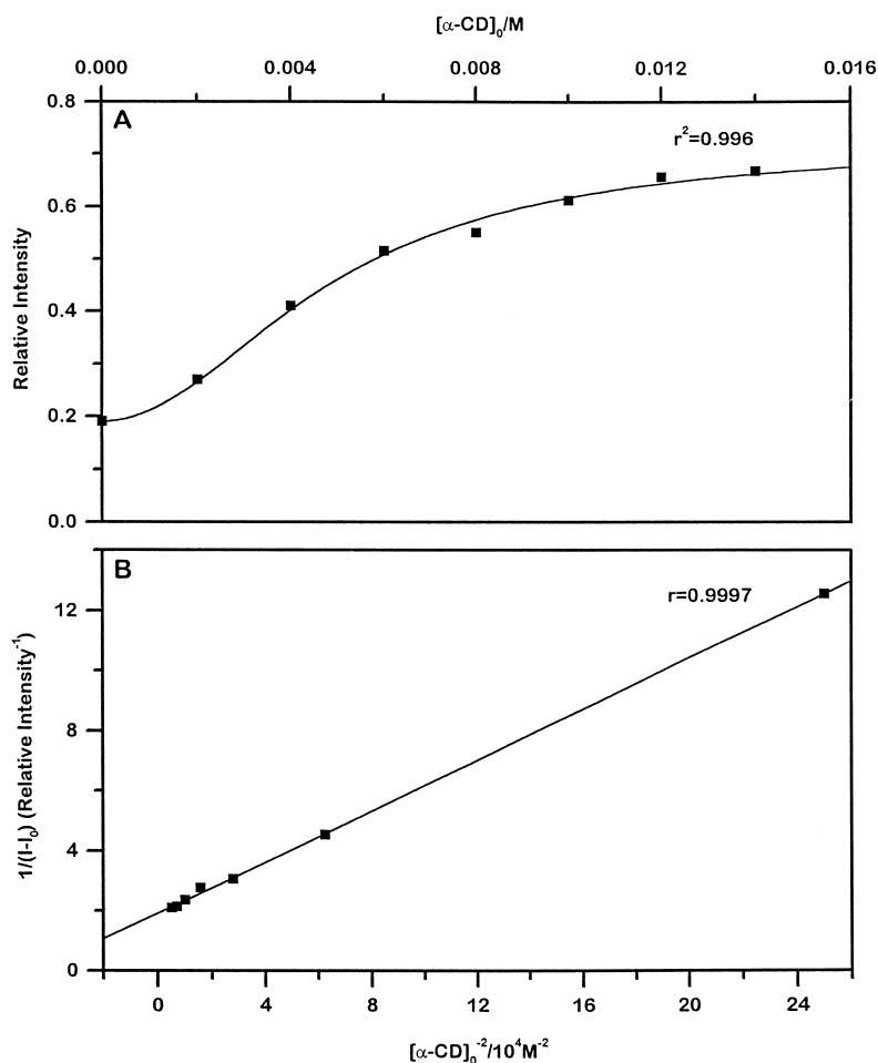
Fig. 5. Plots of the relative fluorescence intensity (A) and 1/(I - I_0) (B) versus [\alpha\text{-CD}]_0 and [\alpha\text{-CD}]_0^2 , respectively, for DBO44BT complexed to \alpha -CD. The full line in (A) is the nonlinear regression fit to the experimental data following Eq. (5).
